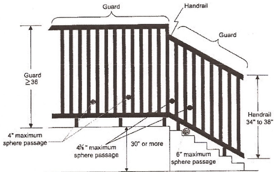
Figure 3.14: Stair Geometry
