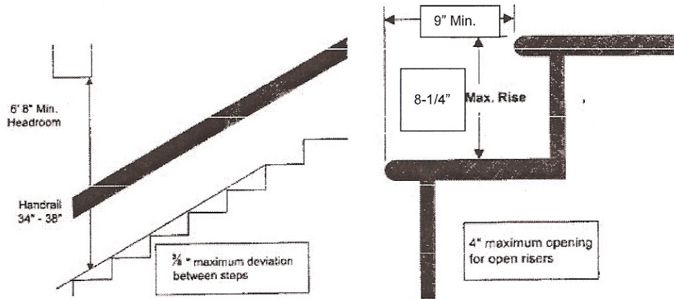
Figure 3.14: Stair Geometry
